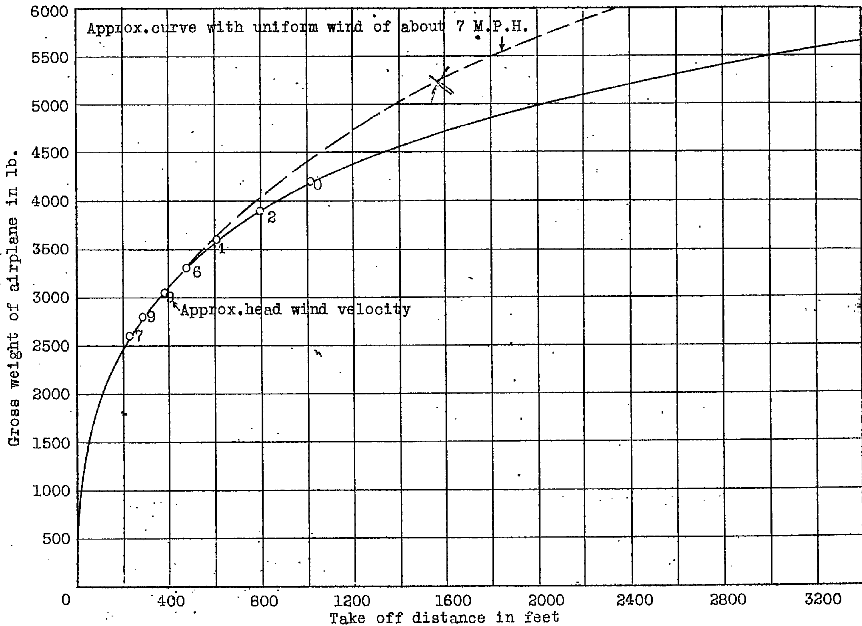
Fig. 8 Take off tests. Altitude of field 600 ft. Ryan NYP airplane.
